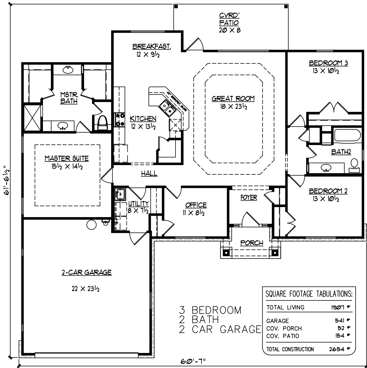
FLOOR PLAN
