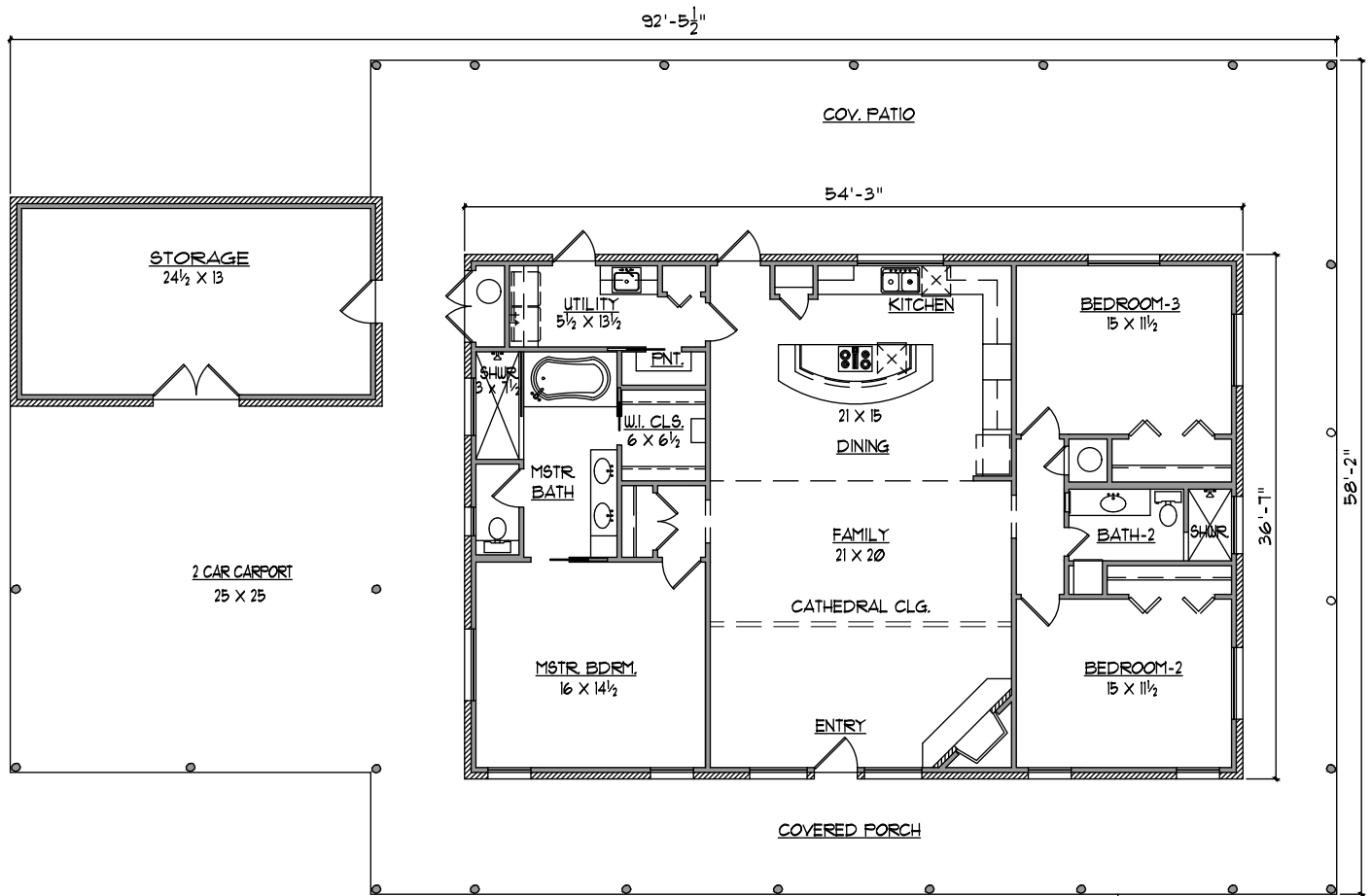
FLOOR PLAN
