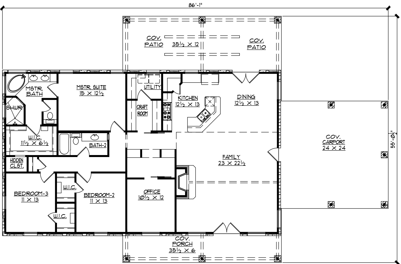
FLOOR PLAN
