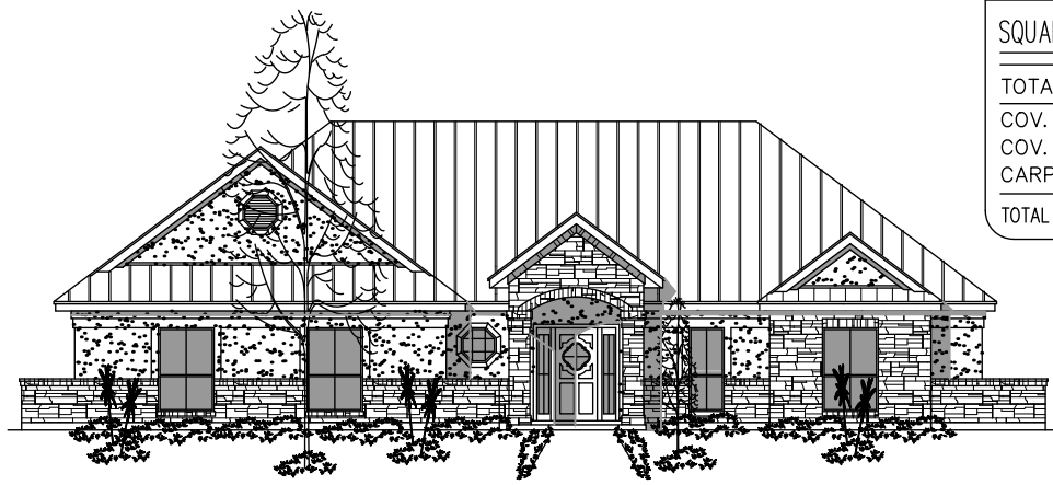
FRONT ELEVATION
