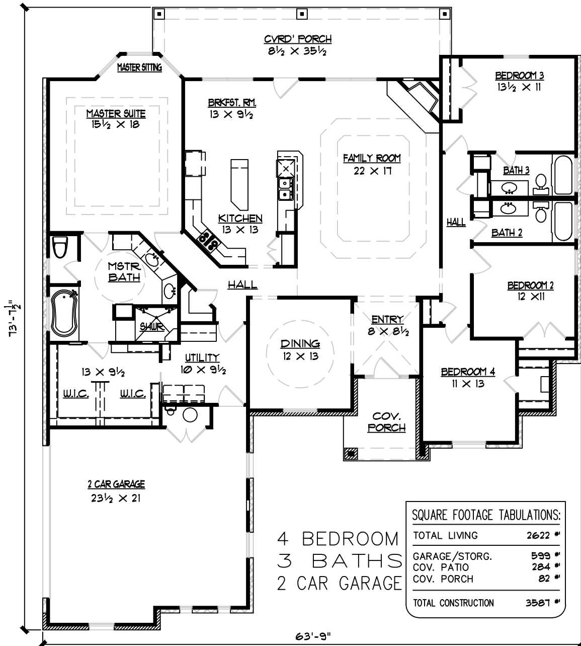
FLOOR PLAN
