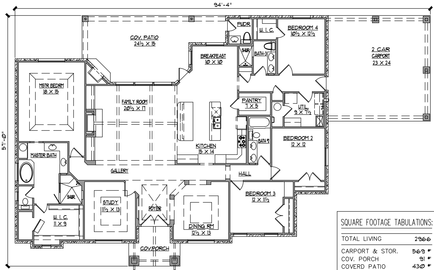
FLOOR PLAN
