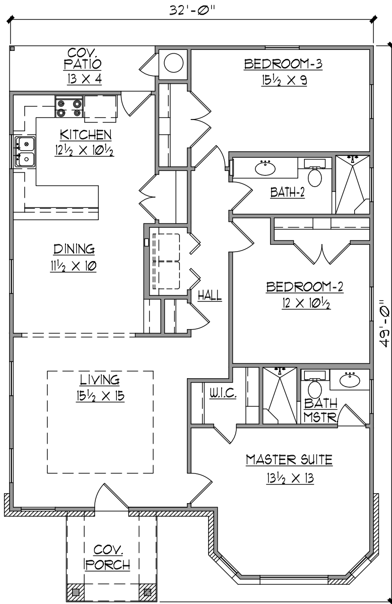
FLOOR PLAN
