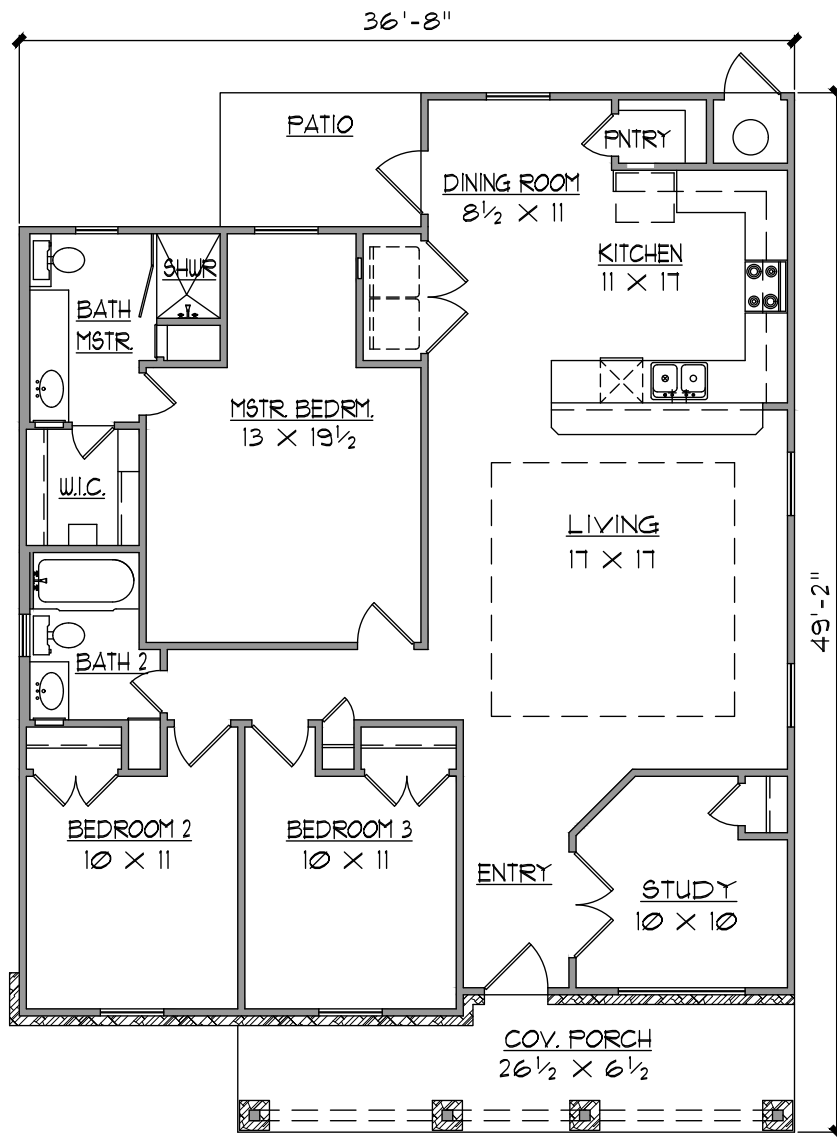
FLOOR PLAN
