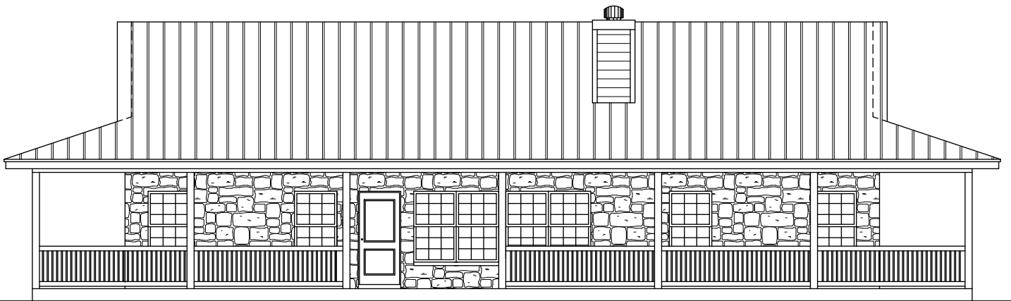
FRONT ELEVATION
