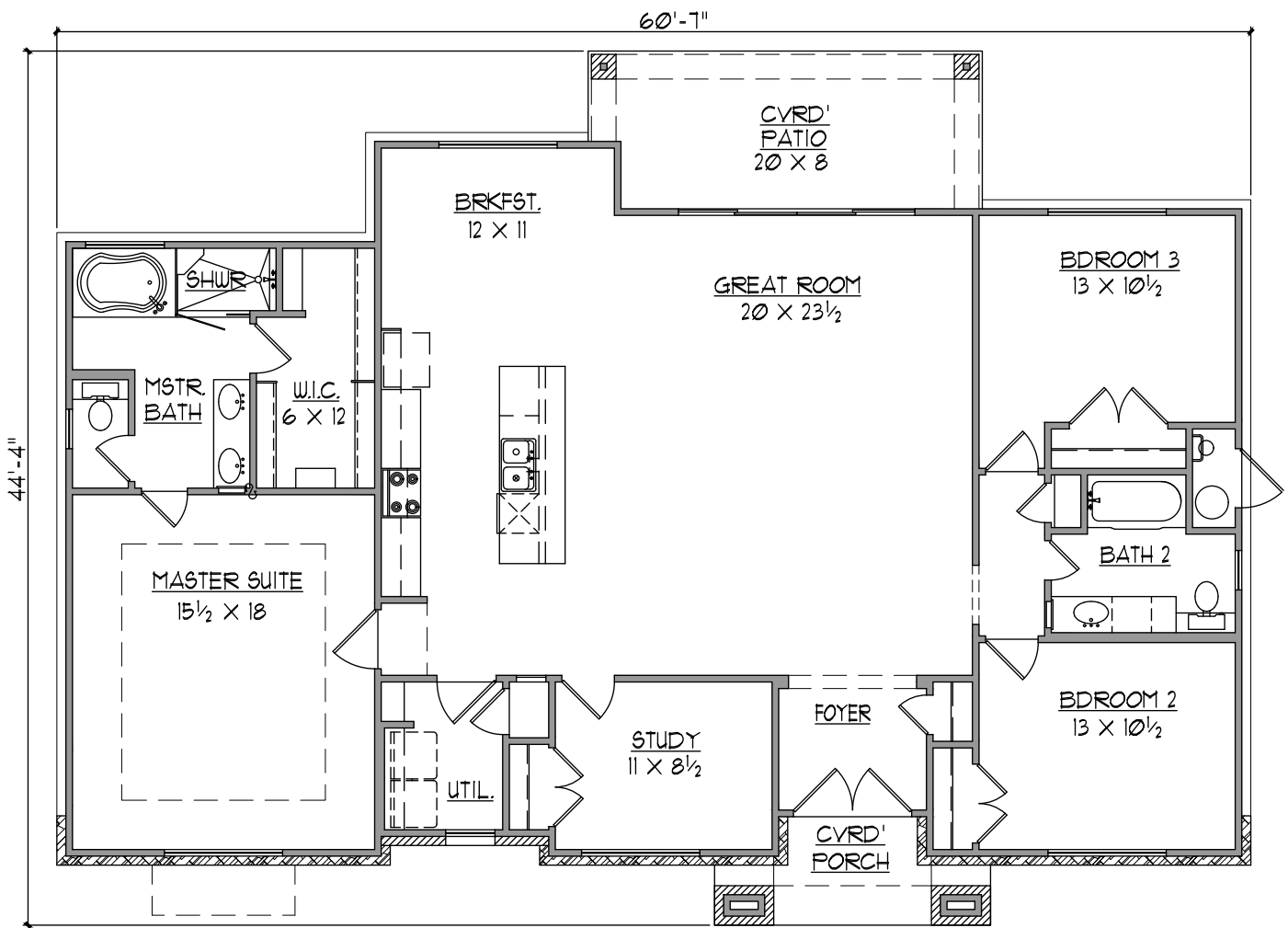
FLOOR PLAN
