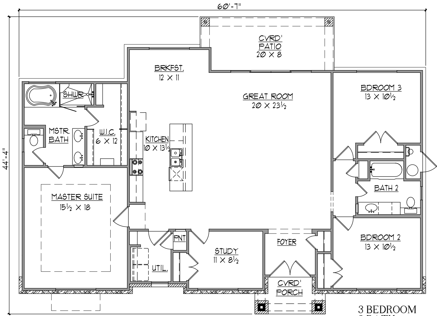
FLOOR PLAN
