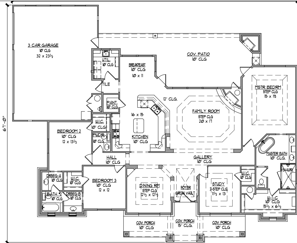
FLOOR PLAN
