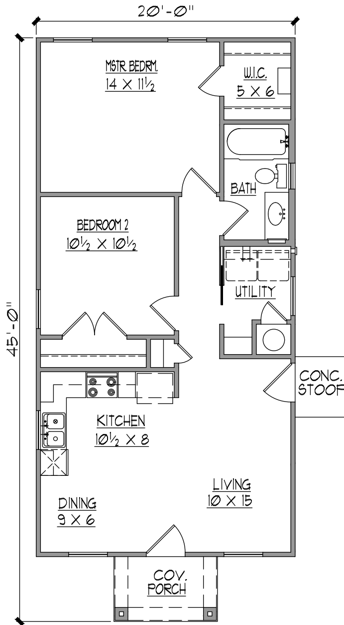
FLOOR PLAN
