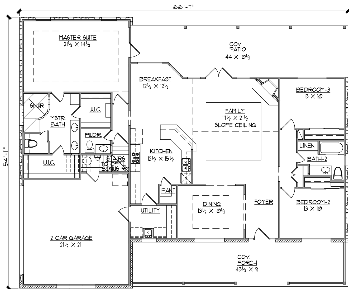
FLOOR PLAN
